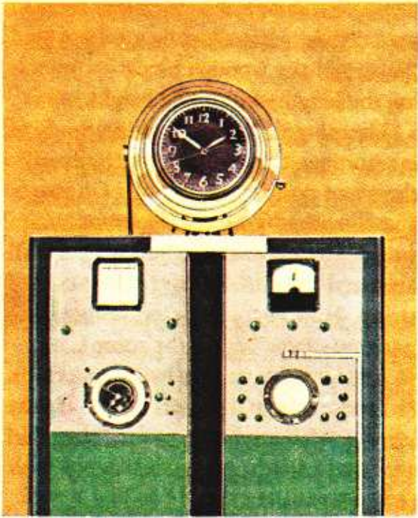
The first Ammonia Atomic Clock was built by the U.S. Bureau of Standards in 1949. The ammonia gas is in the wave guide that is wound around the face of the electric clock. The cabinet, seen only partly here, houses the oscillator and electronic circuits.
